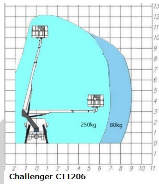
WORKING FLIGHT ENVELOPE
