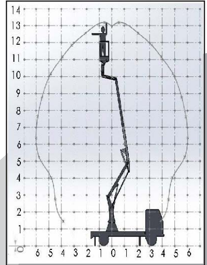
WORKING FLIGHT ENVELOPE
